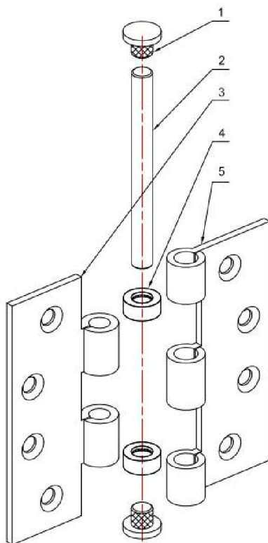
EXPLODED VIEW
