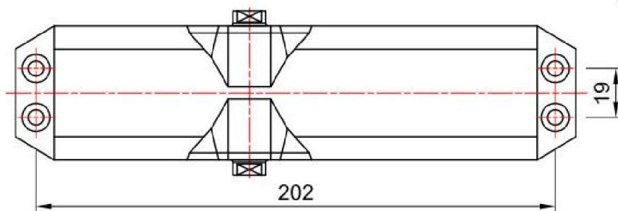
BASE / FIXING VIEW
